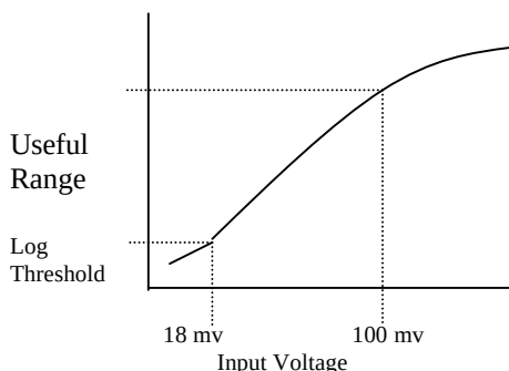
Figure 4. Single Log stage transfer Function
