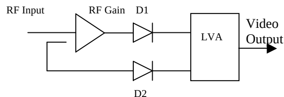
Figure 7. Extended Range DLVA
