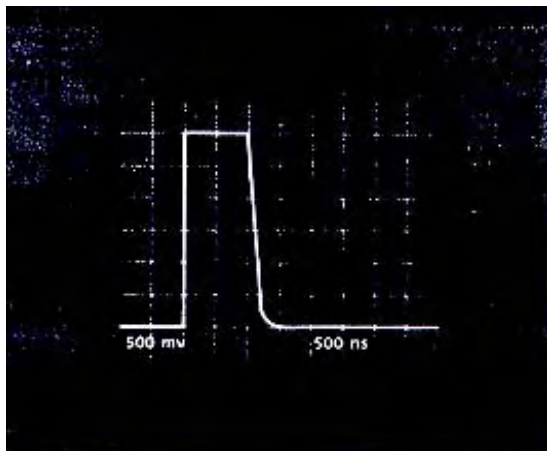
Figure 11 Trailing Edge and Recovery Time
