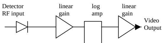
Figure 1. Direct Coupled DLVA Block Diagram
