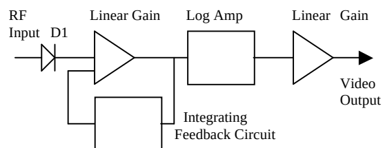
Figure 6. Pseudo AC coupled DLVA
