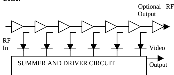
Figure 9 Successive Detection Log Video Amplifier
