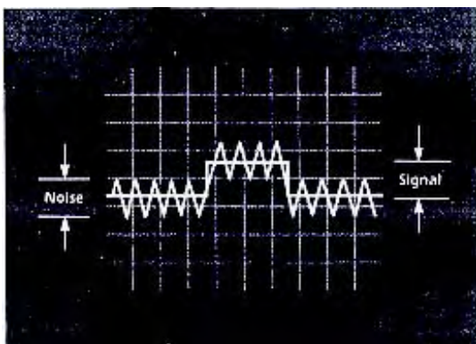
Figure 10. Video Pulse at Tangential Signal Sensitivity
