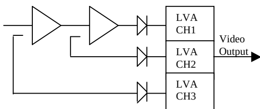
Figure 8. Extended Range DLVA with 3 Detectors
