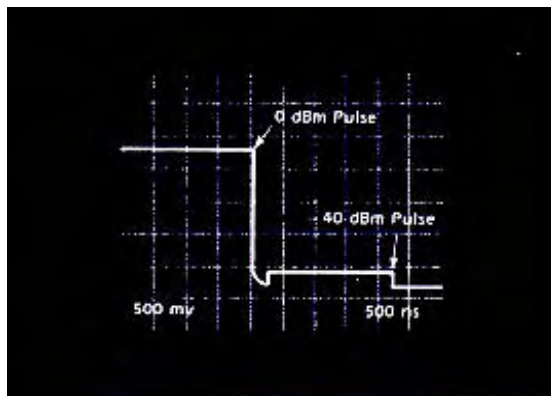
Figure 12. Two Pulse Method of Recovery Time Measurement.
