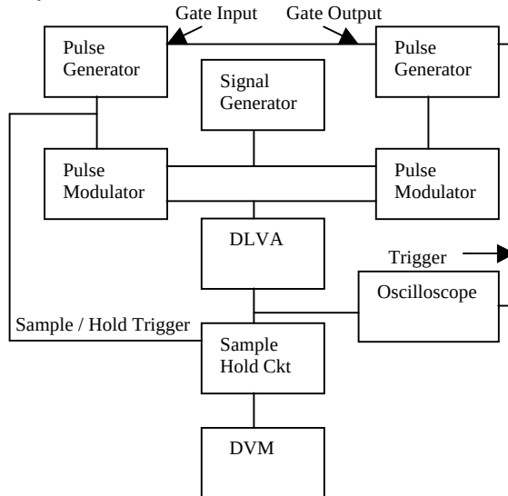
Figure 13 Recovery Time Test Set-up
