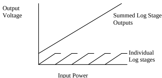
Figure 5. Transfer Response
